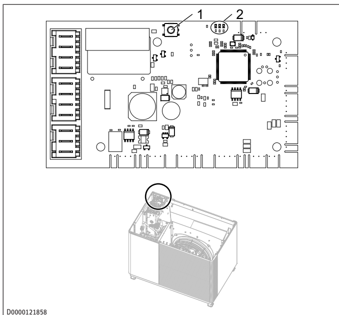
1 Button
