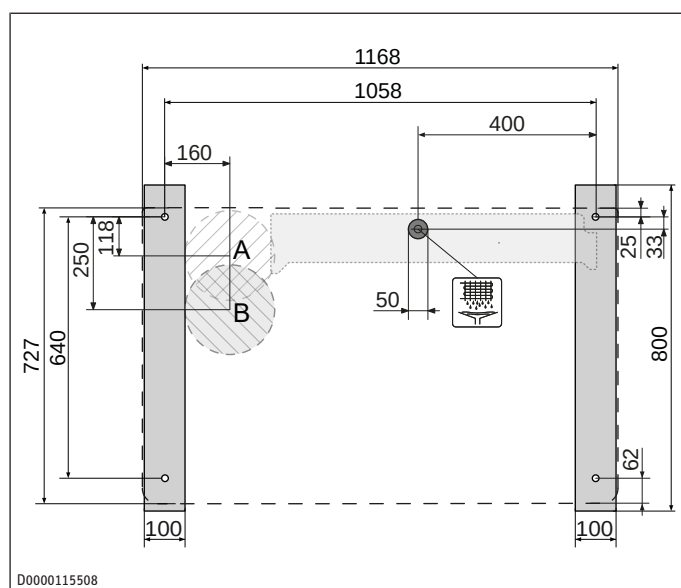
A Hydraulic connections with condensate pan
