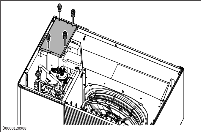
► Loosen the screws for the cover.
