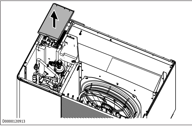
► Remove the cover from the integral heat pump controller (IWS).
